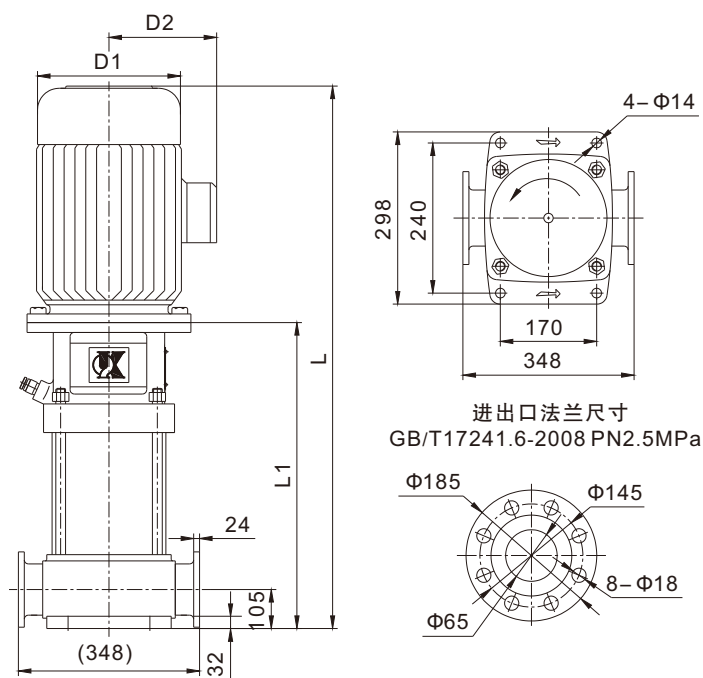
KQDQ65-32
