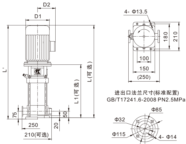
KQDQ25-3
