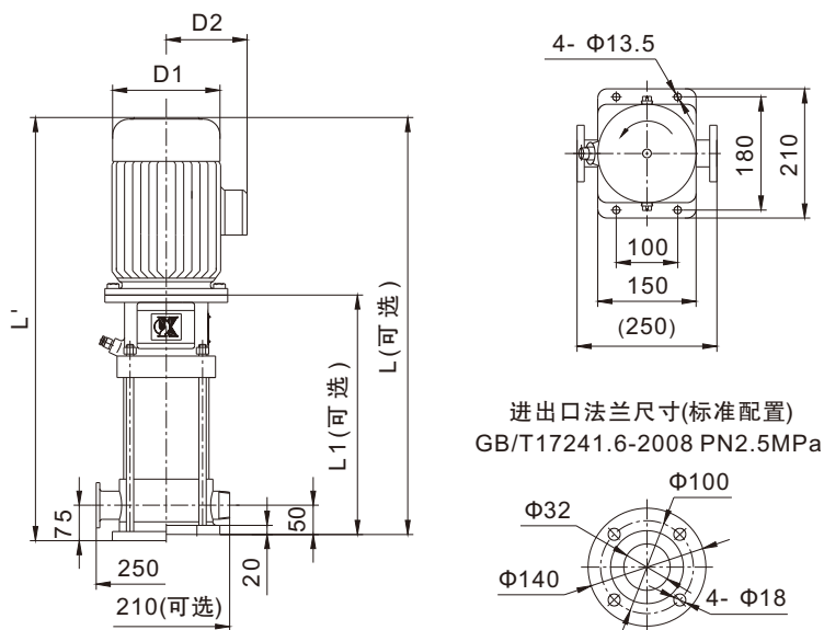
KQDQ32-5
