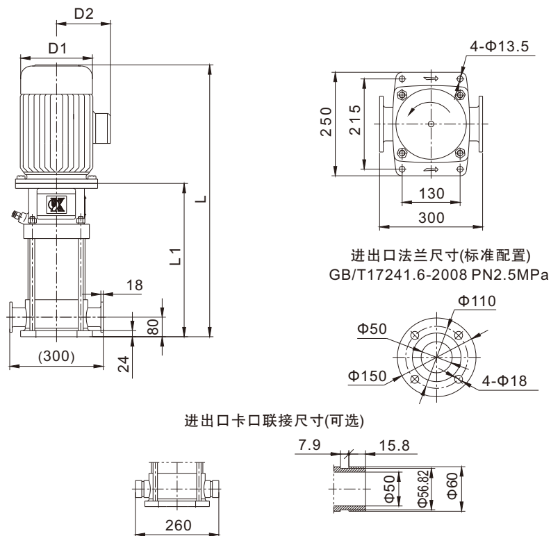
KQDQ40-8
