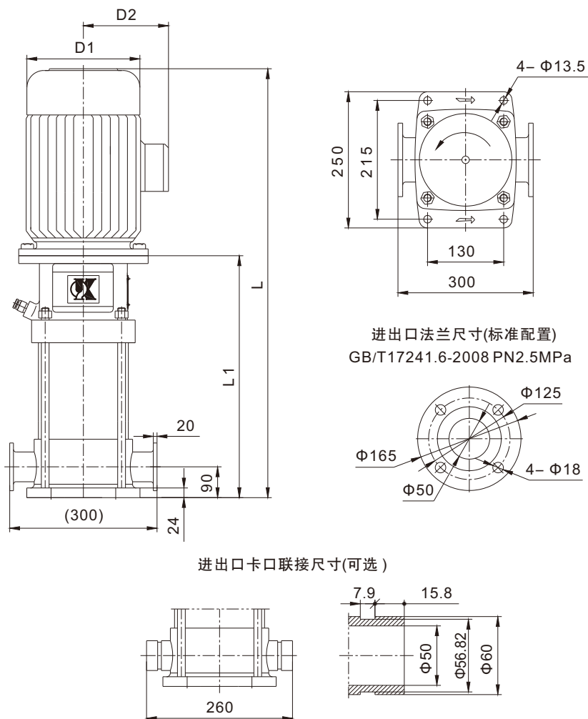
KQDQ50-12
