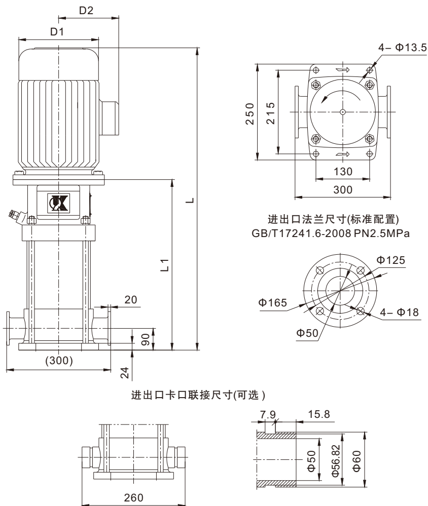
KQDQ50-16
