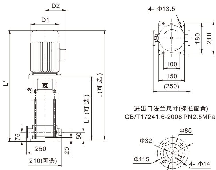
KQDQ25-2
